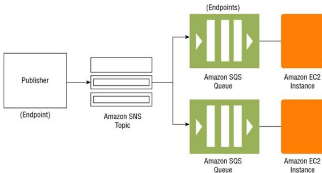
FIGURE 8.5 Diagram of fanout scenario
