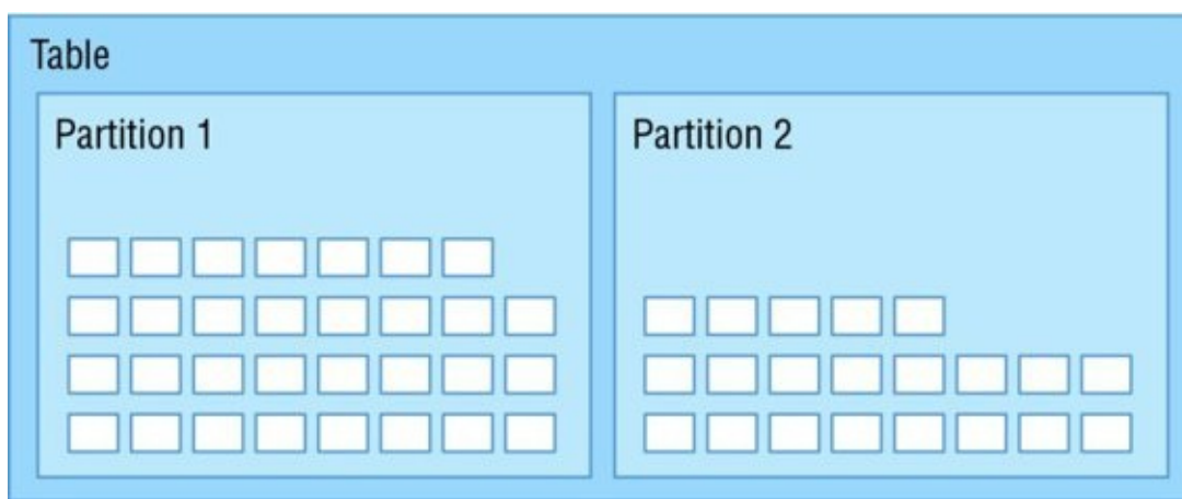
FIGURE 7.4 Table partitioning
