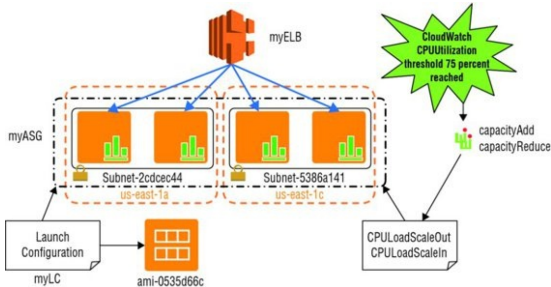
FIGURE 5.3 Amazon CloudWatch alarm triggering scaling out
