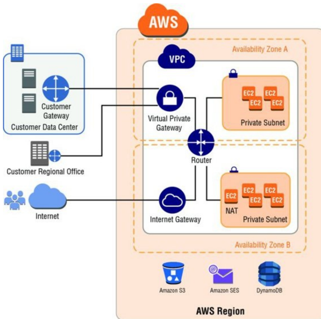
FIGURE 12.5 Amazon VPC network architecture
