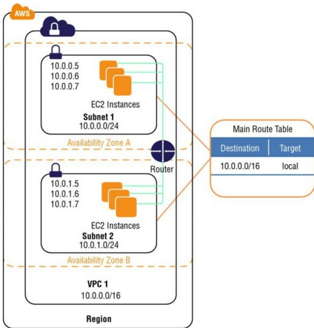
FIGURE 4.1 VPC, subnets, and a route table
