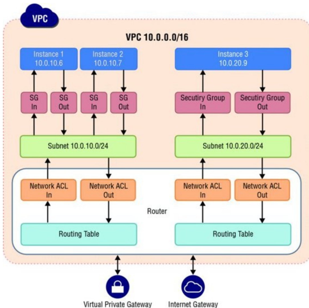
FIGURE 12.6 Flexible network architectures
