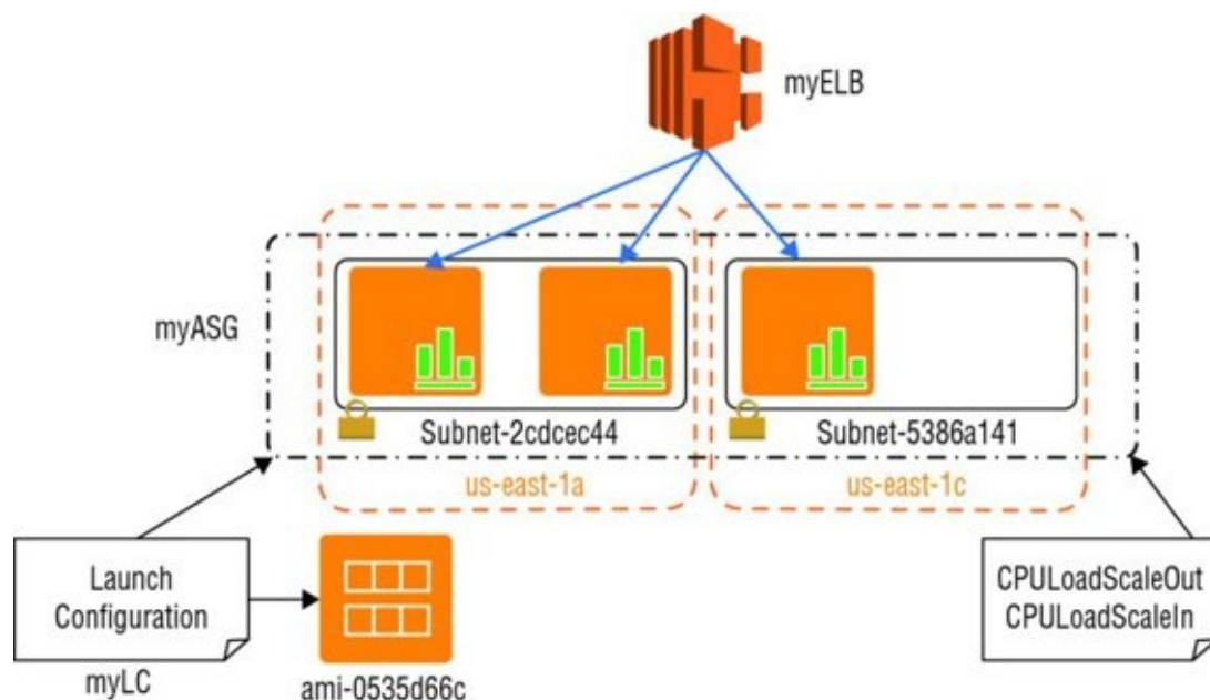
FIGURE 5.2 Auto Scaling group with policy
