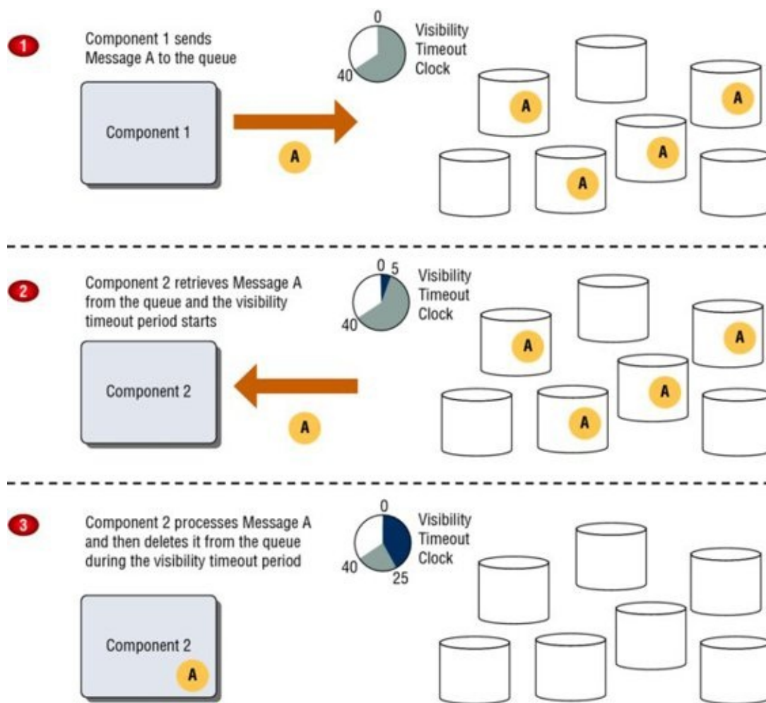
FIGURE 8.1 Message lifecycle
