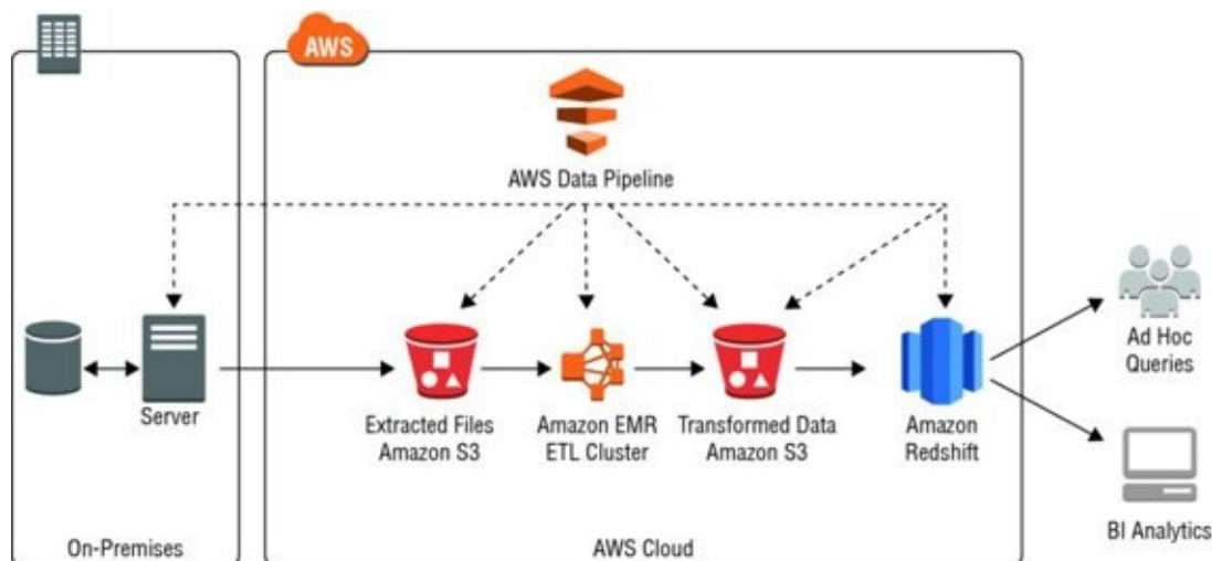
FIGURE 11.5 Example pipeline
