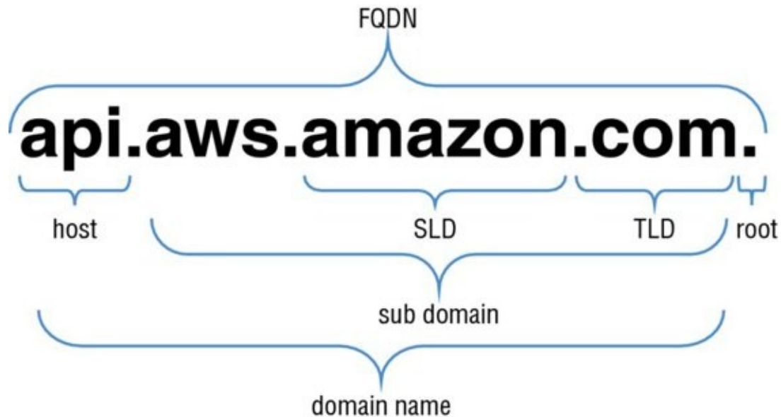
FIGURE 9.1 FQDN components
