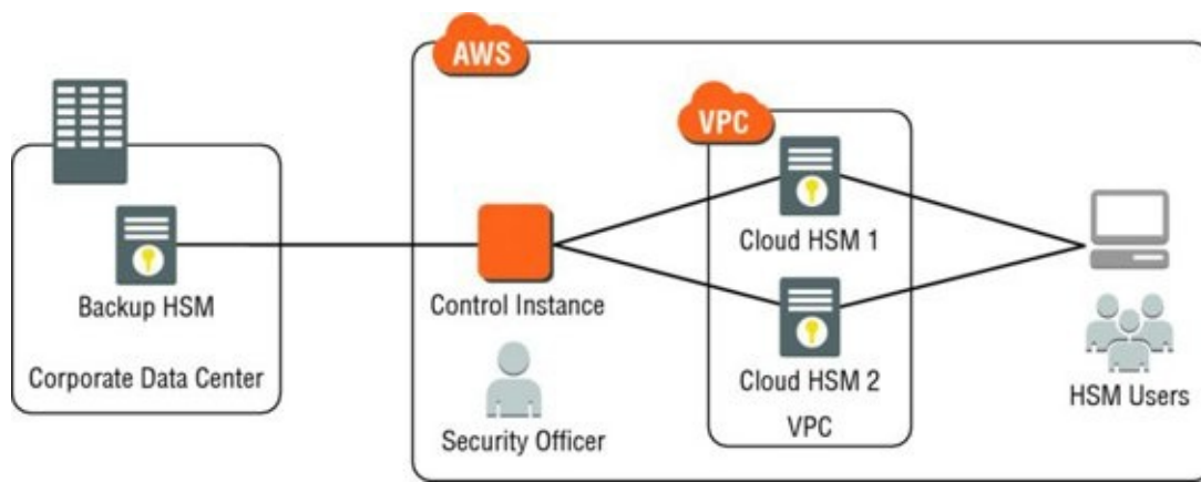
FIGURE 11.2 High availability CloudHSM architecture
